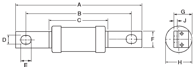
Dimensional Data
