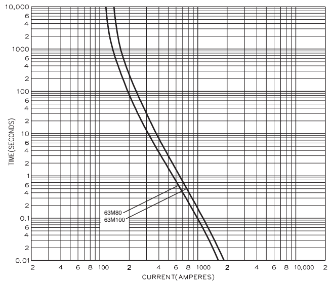
Motor Rated
